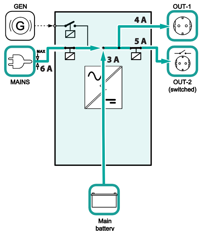
Figure 3-8: Example: The AC-input is limited to 6 A. This is not enough to supply the total load ( 4 + 5 \text{ A} = 9 \text{ A} ) connected to the AC outputs. The inverter will supply the remaining 9 - 6 = 3 \text{ A} .
