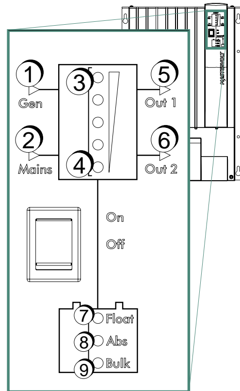
Figure 7-1: Error LEDs
